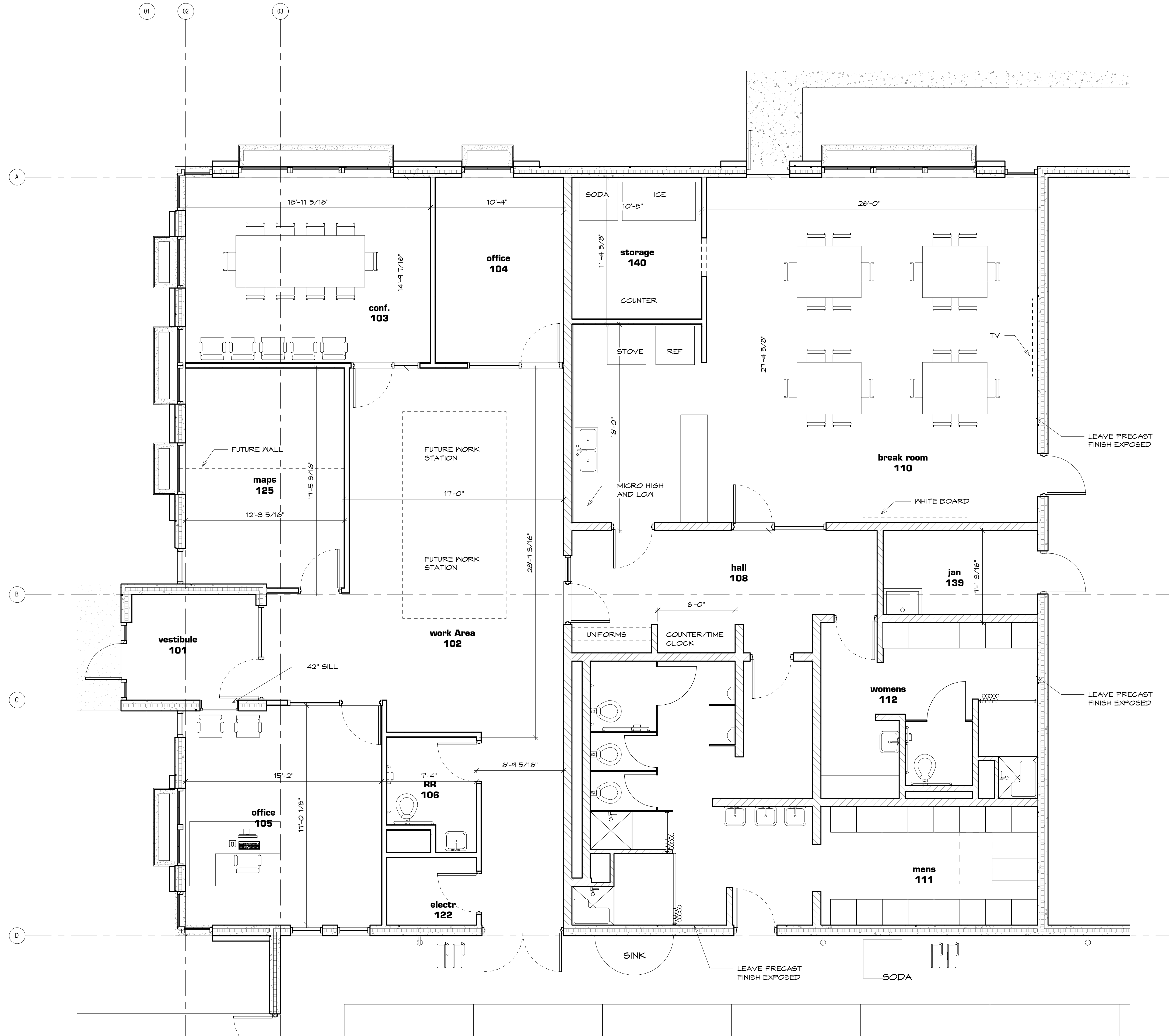
1 Office Floor Plan 1/4" = 1'-0"
